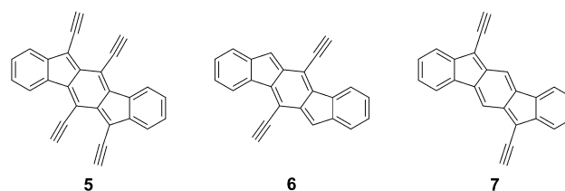
Scheme 2. Calculated ethynylindeno[1,2- b ]fluorene derivatives.
